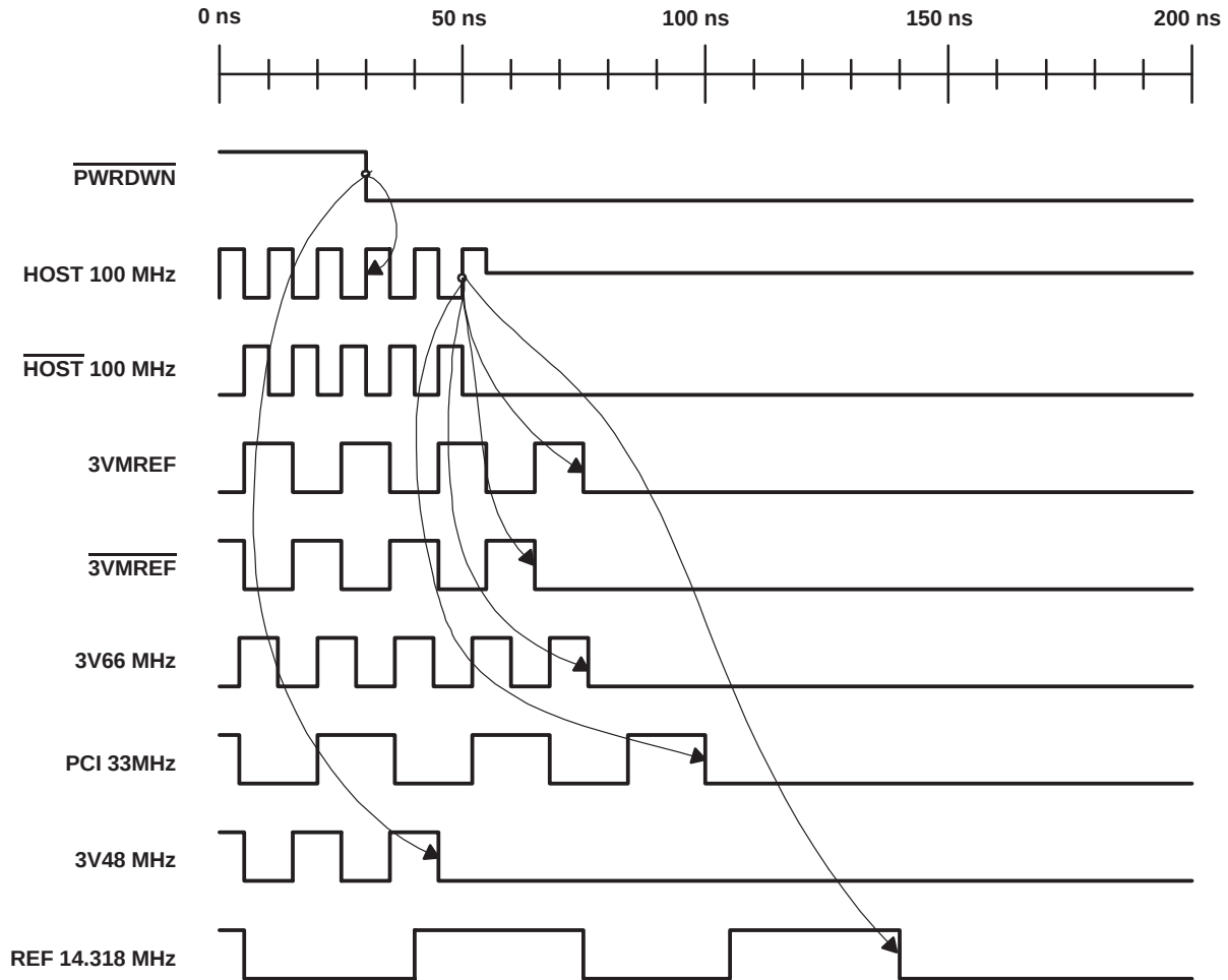
Figure 4. Power \overline{\text{DOWN}} Timing
